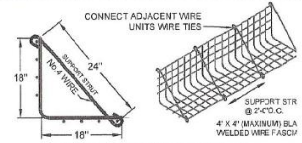
3 WELDED WIRE FABRIC DETAIL SCALE: Not to Scale
