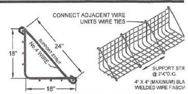
3 WELDED WIRE FABRIC DETAIL SCALE: Not to Scale
