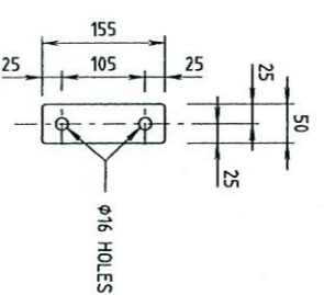
TIE PLATE TYPE T3 CUT FROM 50 x 5 FLAT 344 REQUIRED
