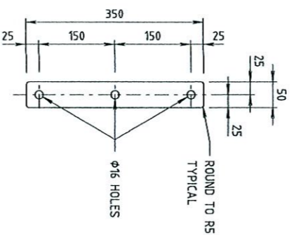
TIE PLATE TYPE T1 CUT FROM 50 x 5 FLAT 344 REQUIRED
